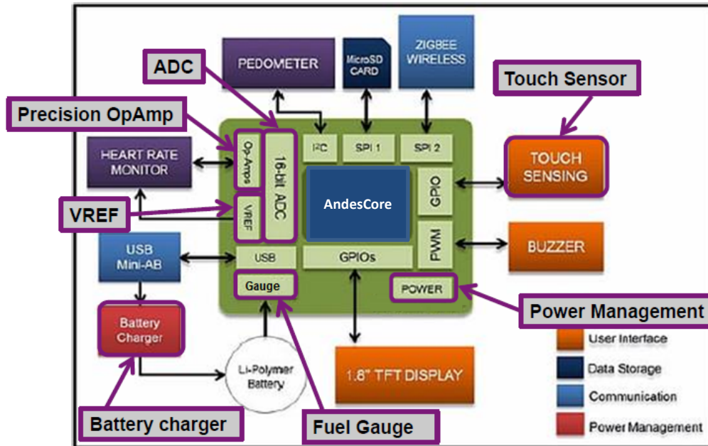
IoT Block Diagram
