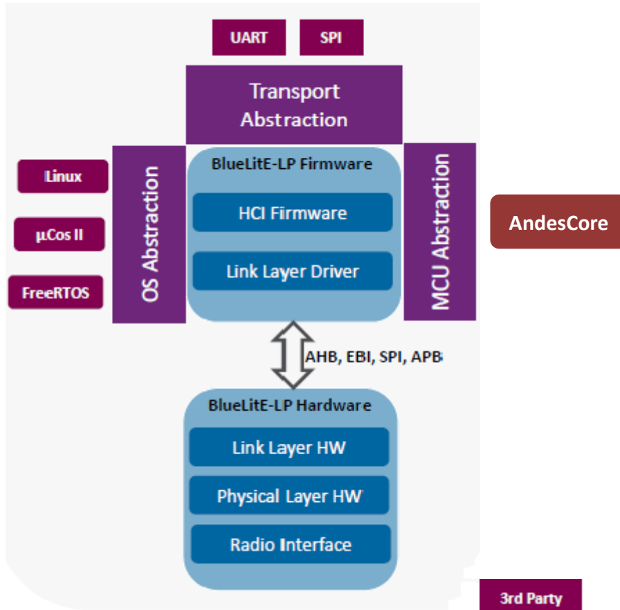
AndesCore Bluetooth Block Diagram
